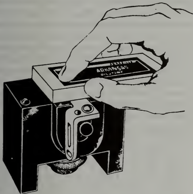
FIGURE 4-66. Using the contact point dressing stone.
